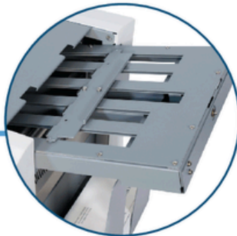
Automatic Fold Plates Simply choose form size and fold type and the plates will adjust automatically
