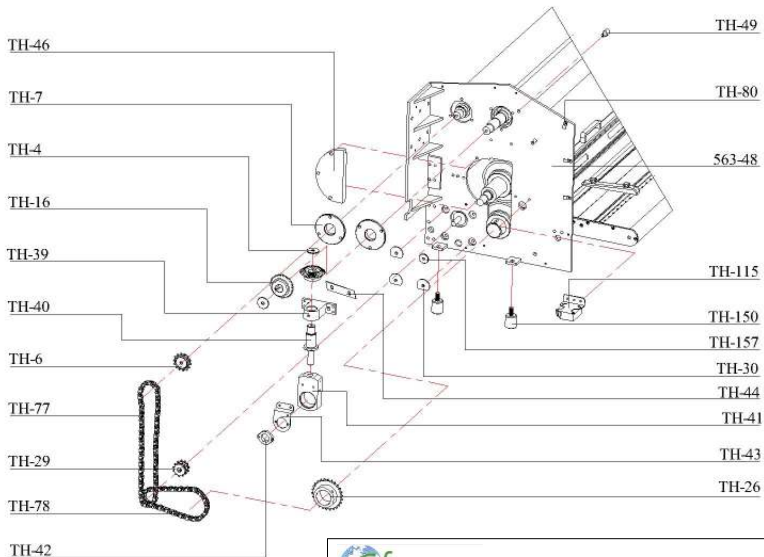
View 7 – Left side plate - Outside
