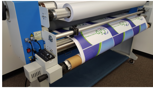
Optional Rear Rewind/Slitter
