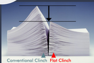
Conventional Clinch
