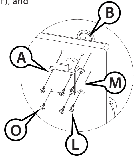
Detail - (C)
