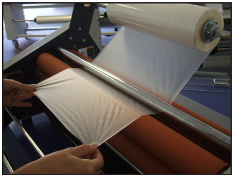
Thread film from top mandrel down under top idler bar and over top laminating roller surface as shown (ensure film is loaded with adhesive side up)
