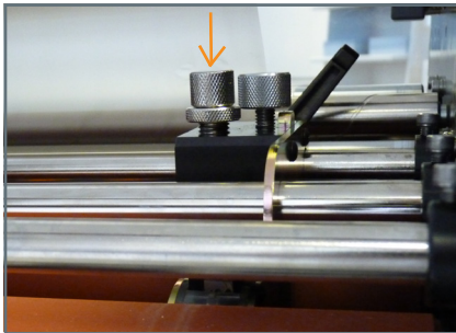
24. Ensure top film perforation wheel is selected. Turn clockwise.
