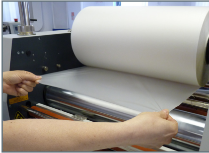
10. Ensure film feeds from the bottom of the roll.
