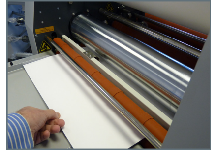
12. Press rubber roller to drop gate and slide in plain print, ensure it goes through anti-curl device and into pull rollers.
