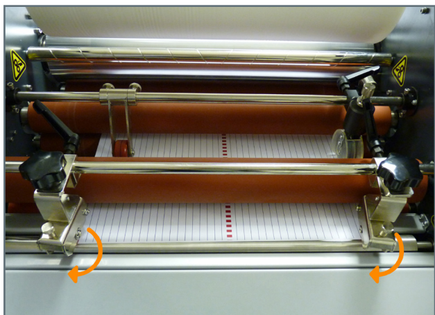
1. Position the wheels on each edge of the laminated sheet as shown.
