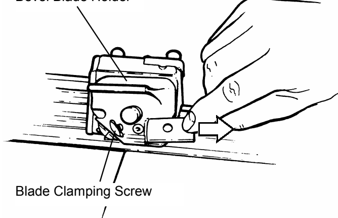
Bevel Blade Holder
